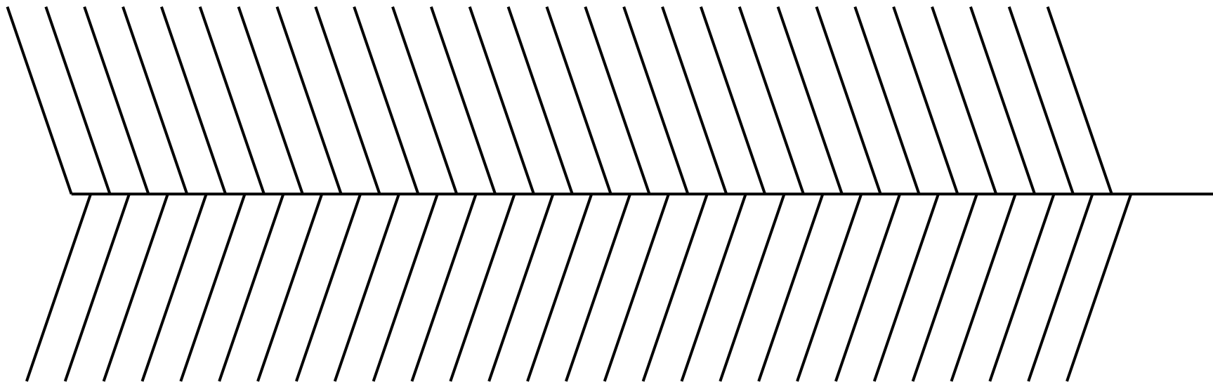
Crosscut handsaw fleam guide (fold on horizontal line) Fleam angle: 20 degrees
